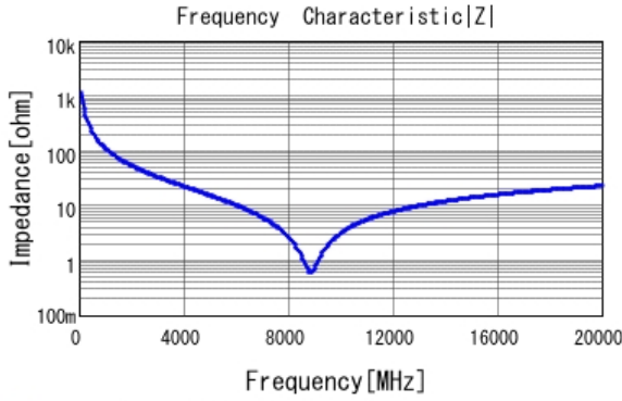
■ GRM0224C1H1R4WA03 |Z| DCOV, 20degC
