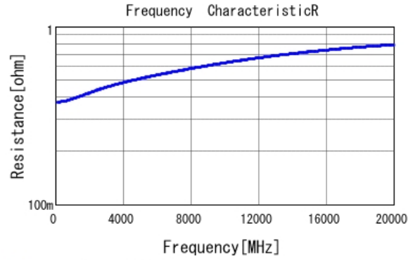
■ GRM0224C1H1R4WA03 R DCOV, 20degC
