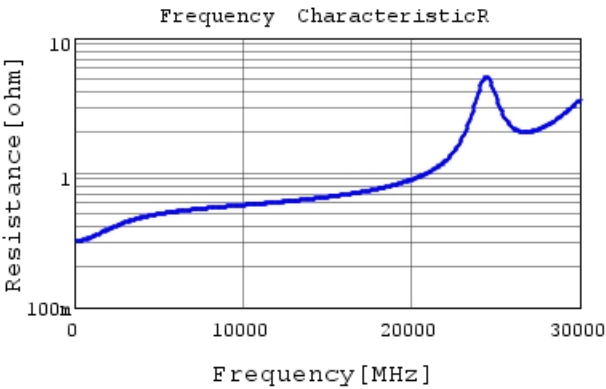
GRM0224C1H1R7BA03 R DCOV,20degC
