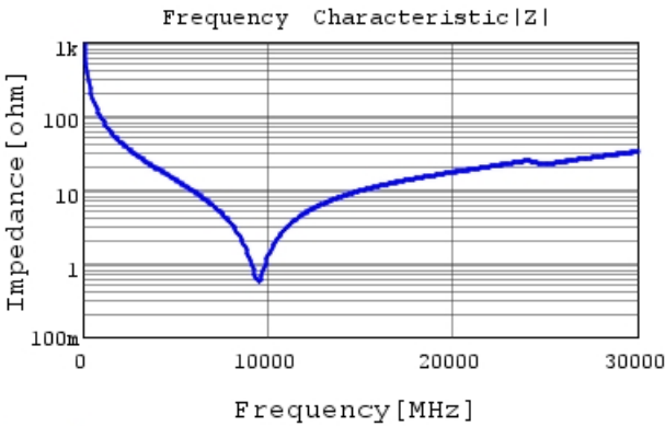
GRM0224C1H1R7BA03 |Z| DCOV,20degC
