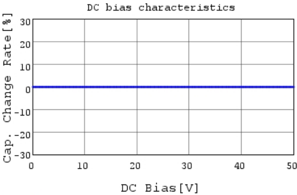
GRM0224C1H1R7BA03 C-DC bias capchange, 20.0
