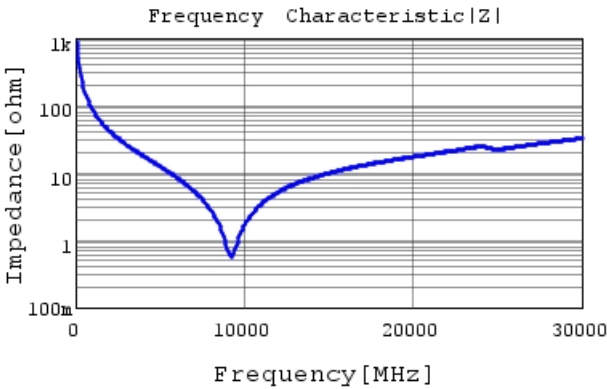
GRM0224C1H1R8BA03 |Z| DCOV,20degC
