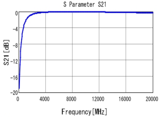
■ GRM0224C1H1R8CA03 S21 DCOV, 20degC
