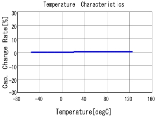
■ GRM0224C1H1R8CA03 C-Temp. capchange, DCOV, AC1Vrms
