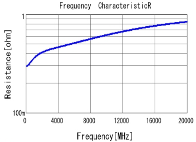
■ GRM0224C1H1R8CA03 R DC0V, 20degC
