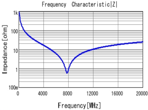
■ GRM0224C1H1R8CA03 |Z| DC0V, 20degC
