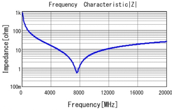
■ GRM0224C1H1R9BA03 |Z| DCOV, 20degC
