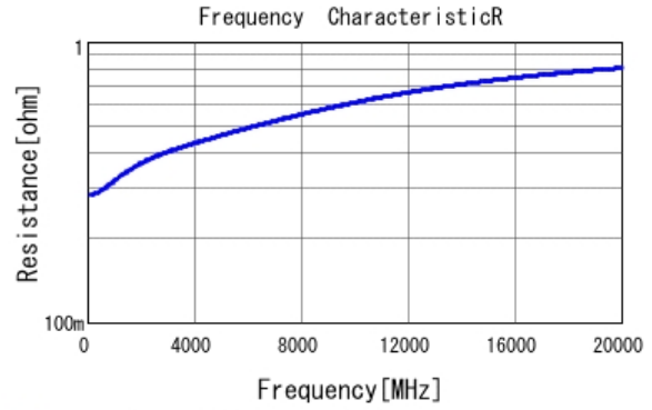
■ GRM0224C1H1R9BA03 R DCOV, 20degC
