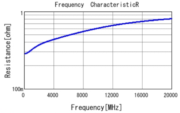
■ GRM0224C1H1R9WA03 R DCOV, 20degC
