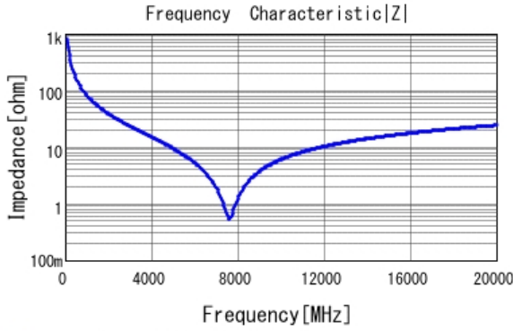
■ GRM0224C1H1R9WA03 |Z| DCOV, 20degC
