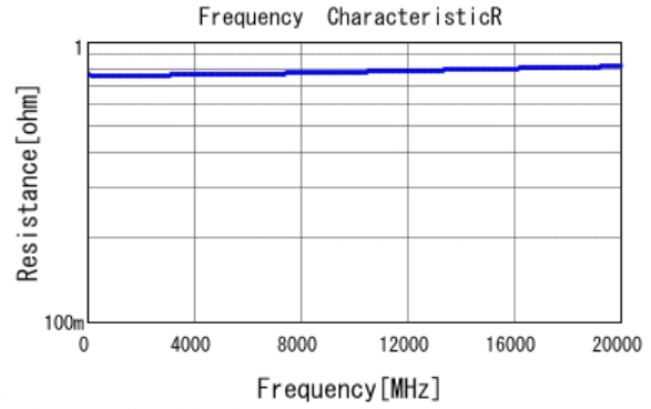
■ GRM0224C1HR30BA03 R DCOV, 20degC
