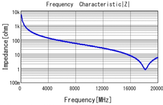
■ GRM0224C1HR30BA03 |Z| DCOV, 20degC
