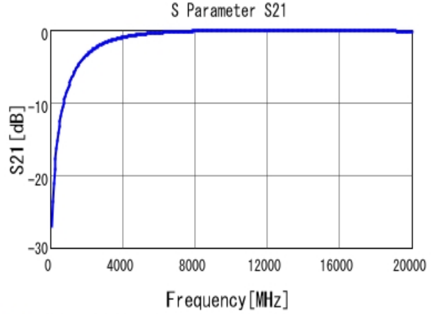
■ GRM0224C1HR70BA03 S21 DCOV, 20degC
