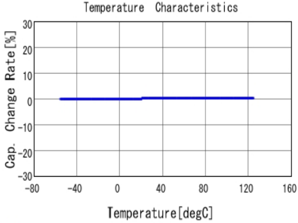
■ GRM0224C1HR70BA03 C-Temp. capchange, DCOV, AC1Vrms
