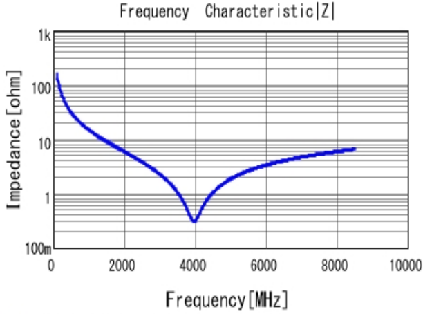
■ GRM0225C1H100GA03 |Z| DCOV, 25degC
