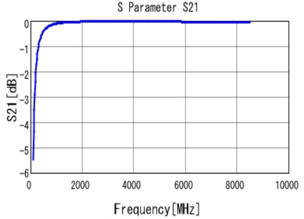
■ GRM0225C1H100GA03 S21 DCOV, 25degC
