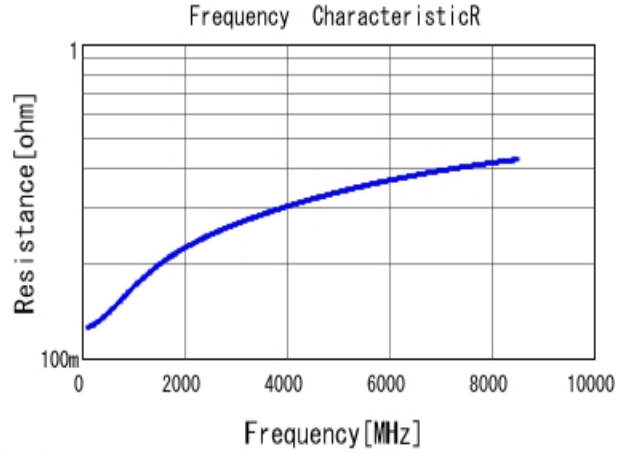
■ GRM0225C1H100GA03 R DCOV, 25degC
