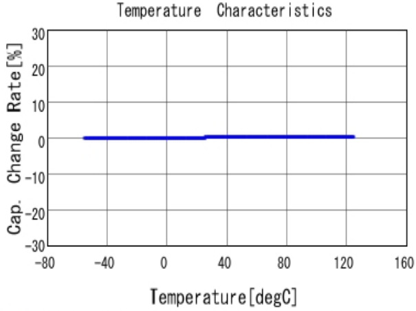
■ GRM0225C1H100GA03 C-Temp. capchange, DCOV, AC1Vrms
