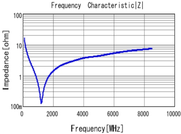
■ GRM0225C1H101JA02 |Z| DC0V, 25degC
