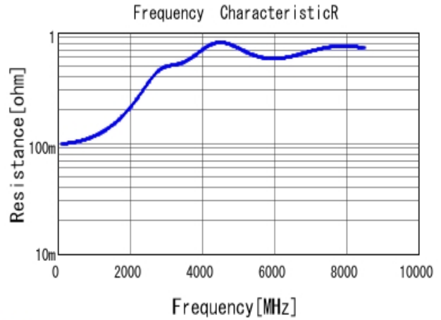
■ GRM0225C1H101JA02 R DC0V, 25degC
