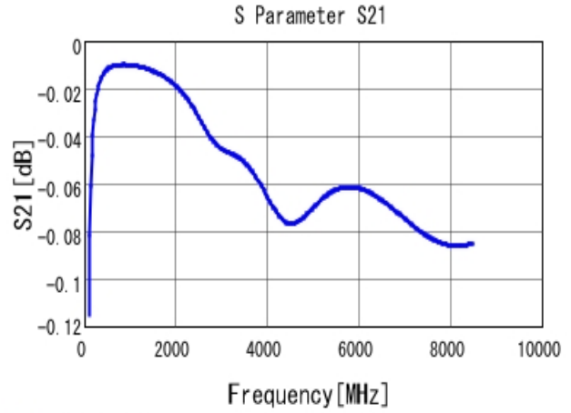
■ GRM0225C1H101JA02 S21 DCOV, 25degC
