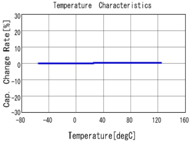
■ GRM0225C1H101JA02 C-Temp. capchange, DCOV, AC1Vrms
