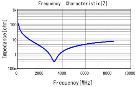
■ GRM0225C1H150JA03 |Z| DCOV, 25degC
