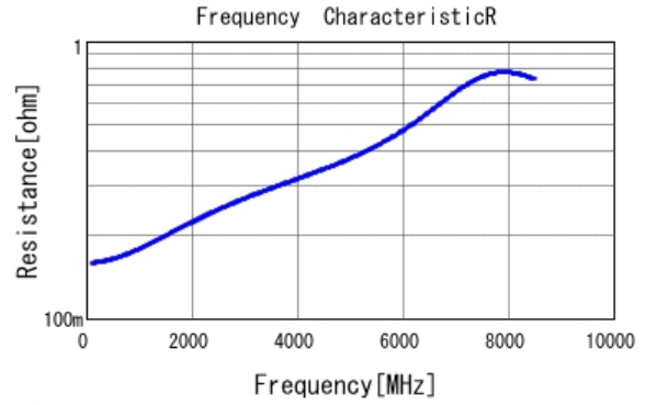
■ GRM0225C1H150JA03 R DCOV, 25degC
