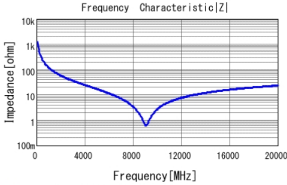
■ GRM0225C1H1R3WA03 |Z| DCOV, 25degC
