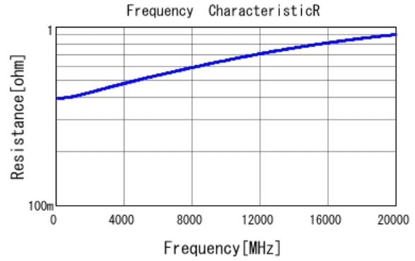
■ GRM0225C1H1R3WA03 R DCOV, 25degC
