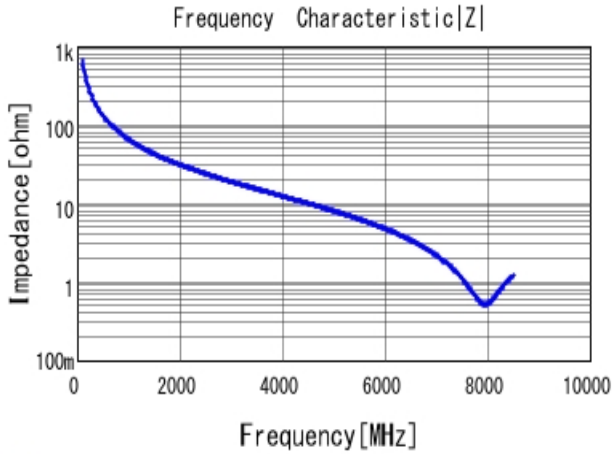
■ GRM0225C1H2R4BA03 |Z| DC0V, 25degC
