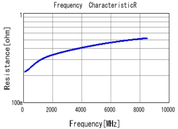
■ GRM0225C1H2R4BA03 R DC0V, 25degC
