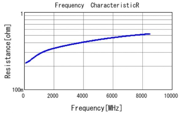
■ GRM0225C1H2R5CA03 R DCOV, 25degC
