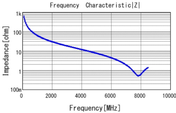
■ GRM0225C1H2R5CA03 |Z| DCOV, 25degC
