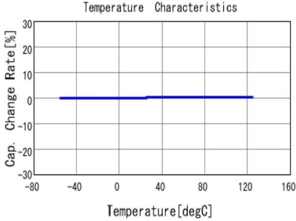
■ GRM0225C1H2R7CA03 C-Temp. capchange, DCOV, AC1Vrms
