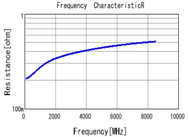
■ GRM0225C1H2R7CA03 R DC0V, 25degC
