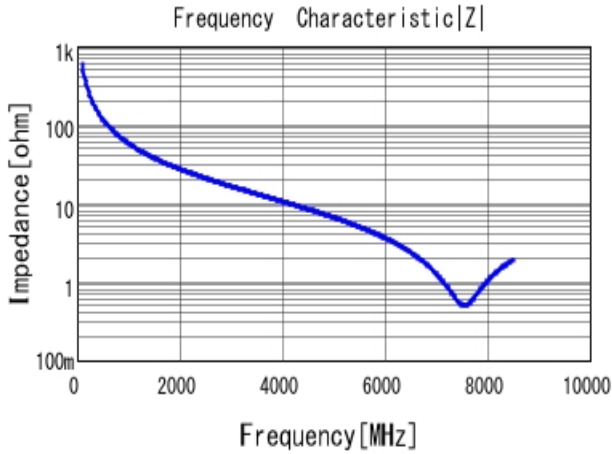
■ GRM0225C1H2R7CA03 |Z| DC0V, 25degC
