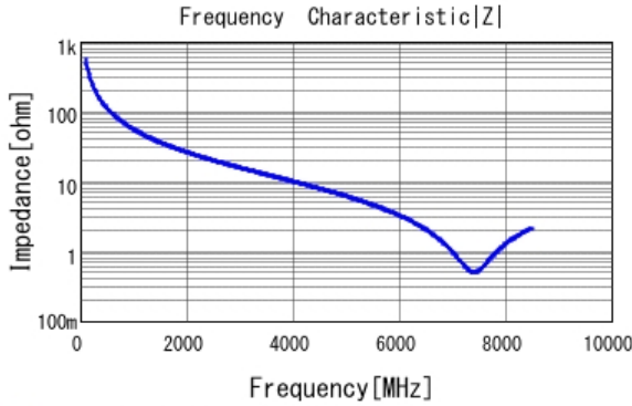
■ GRM0225C1H2R8WA03 |Z| DCOV, 25degC
