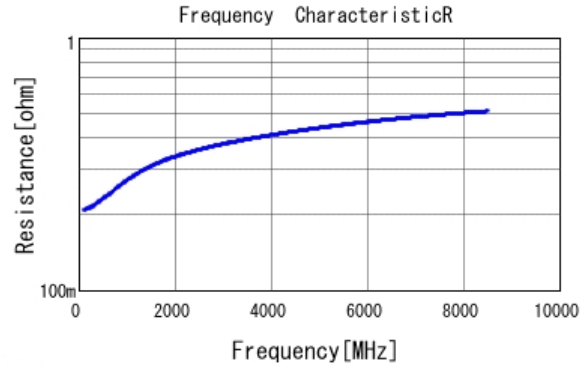
■ GRM0225C1H2R8WA03 R DCOV, 25degC
