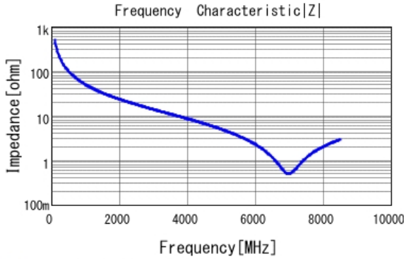
■ GRM0225C1H3R1BA03 |Z| DCOV, 25degC
