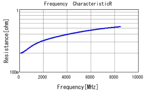
■ GRM0225C1H3R1BA03 R DCOV, 25degC
