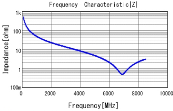
■ GRM0225C1H3R2WA03 |Z| DCOV, 25degC
