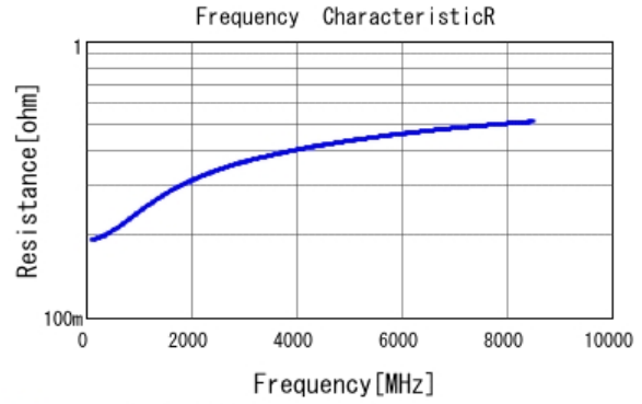
■ GRM0225C1H3R2WA03 R DCOV, 25degC
