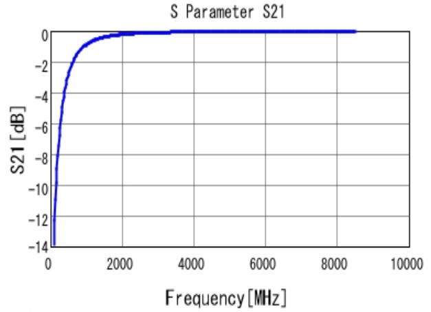
■ GRM0225C1H3R3CA03 S21 DCOV, 25degC
