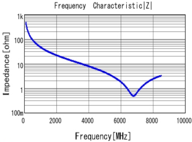
■ GRM0225C1H3R3CA03 |Z| DC0V, 25degC
