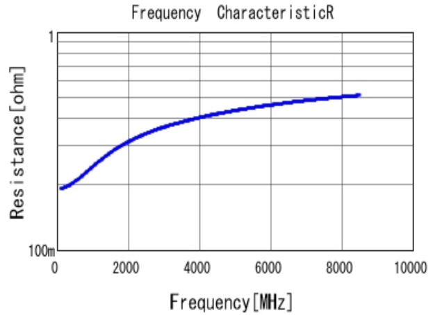
■ GRM0225C1H3R3CA03 R DC0V, 25degC
