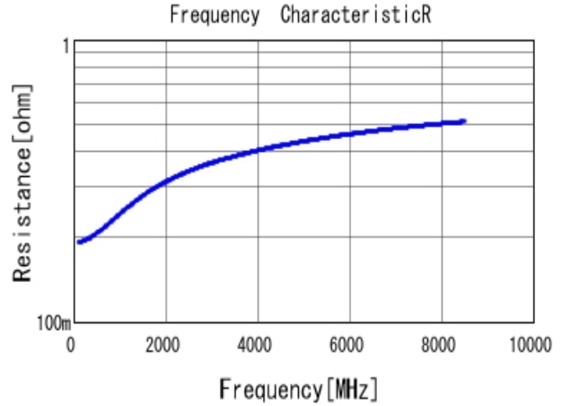
■ GRM0225C1H3R4BA03 R DC0V, 25degC
