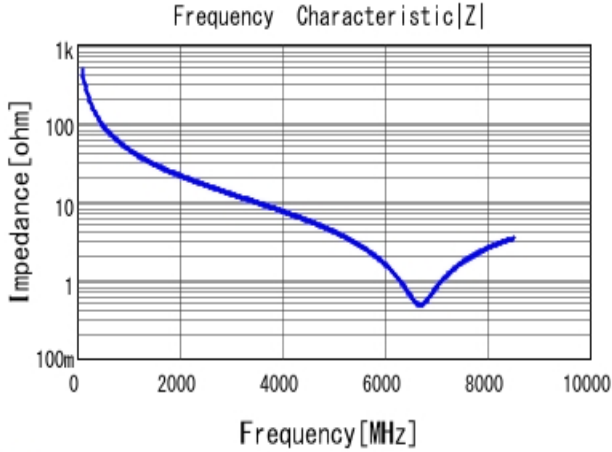
■ GRM0225C1H3R4BA03 |Z| DC0V, 25degC
