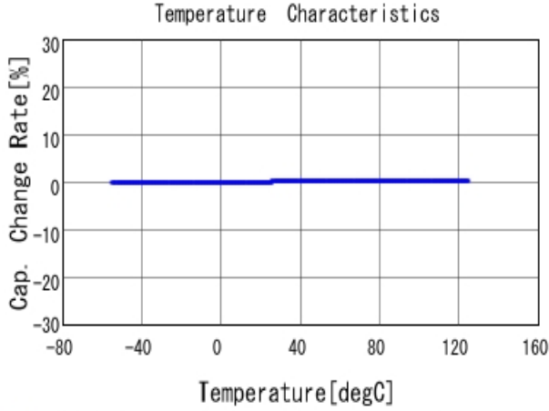
■ GRM0225C1H3R4CA03 C-Temp. capchange, DCOV, AC1Vrms
