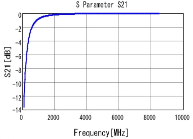
■ GRM0225C1H3R4CA03 S21 DCOV, 25degC
