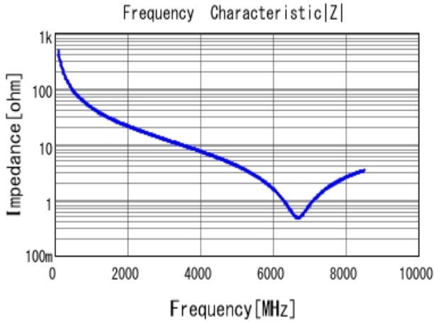
■ GRM0225C1H3R4CA03 |Z| DC0V, 25degC
