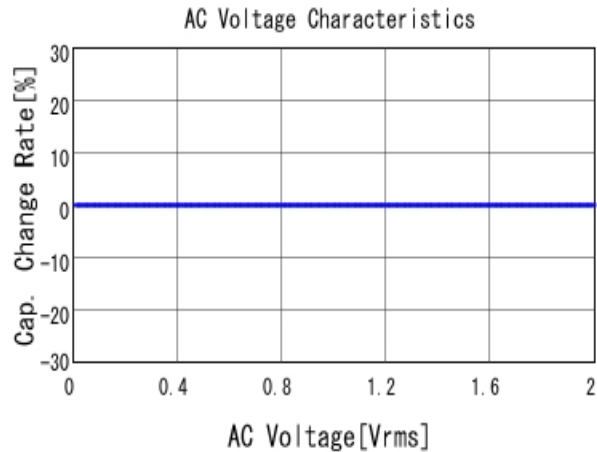
■ GRM0225C1H3R4CA03 C-AC Voltage capchange, DC0V, 25.0d
