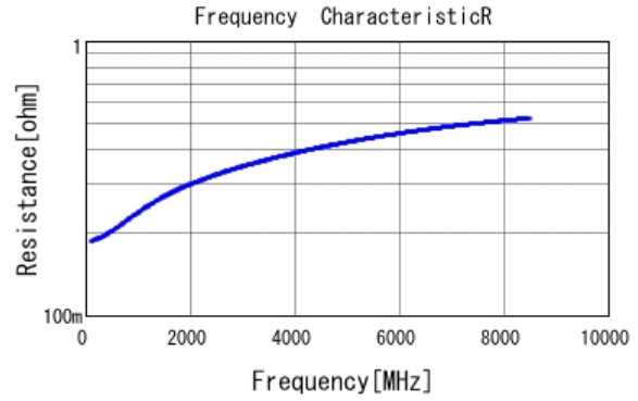
■ GRM0225C1H3R6BA03 R DCOV, 25degC
