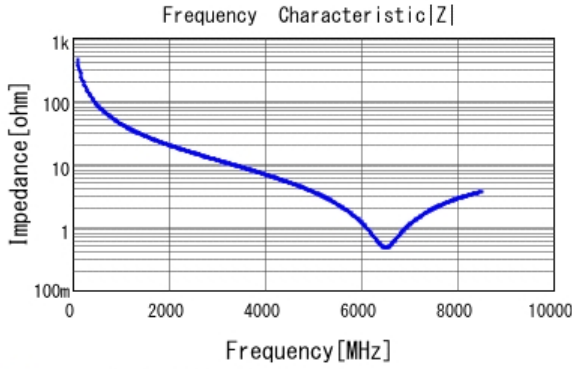
■ GRM0225C1H3R6BA03 |Z| DCOV, 25degC
