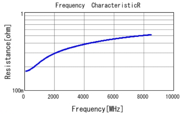
■ GRM0225C1H3R9BA03 R DCOV, 25degC
