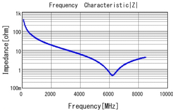
■ GRM0225C1H3R9BA03 |Z| DCOV, 25degC
