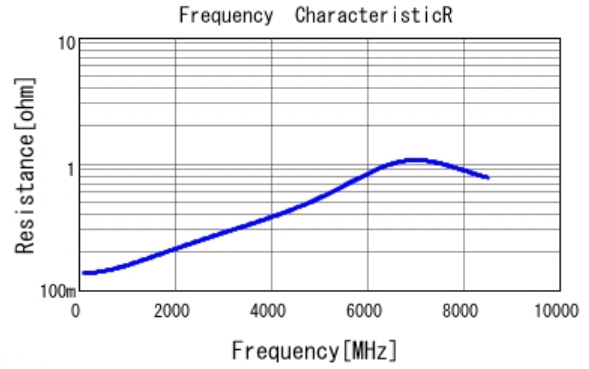
■ GRM0225C1H470JA02 R DCOV, 25degC
