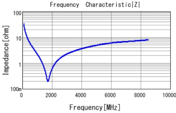
■ GRM0225C1H470JA02 |Z| DCOV, 25degC
