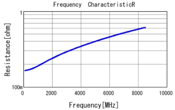
■ GRM0225C1H4R1BA03 R DCOV, 25degC
