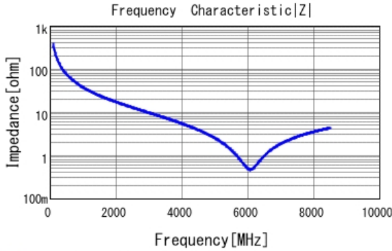
■ GRM0225C1H4R1BA03 |Z| DCOV, 25degC
