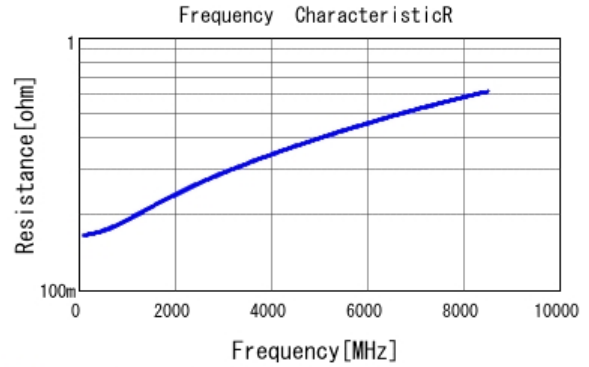
■ GRM0225C1H4R2CA03 R DCOV, 25degC
