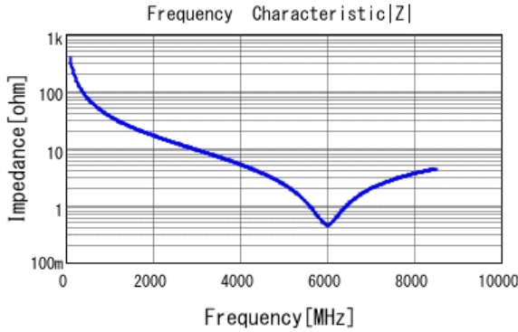
■ GRM0225C1H4R2CA03 |Z| DCOV, 25degC
