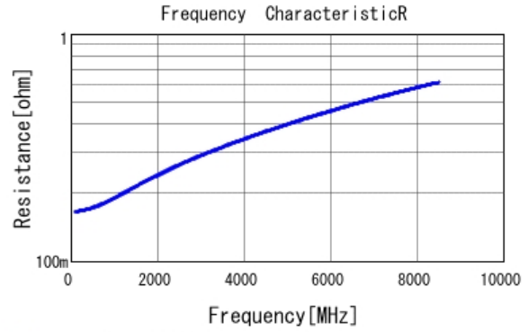
■ GRM0225C1H4R3BA03 R DCOV, 25degC
