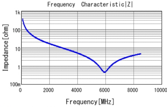
■ GRM0225C1H4R3BA03 |Z| DCOV, 25degC
