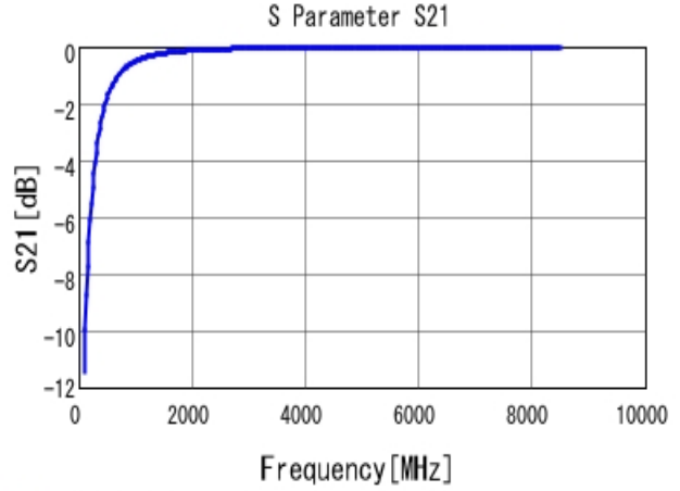
■ GRM0225C1H4R4CA03 S21 DCOV, 25degC
