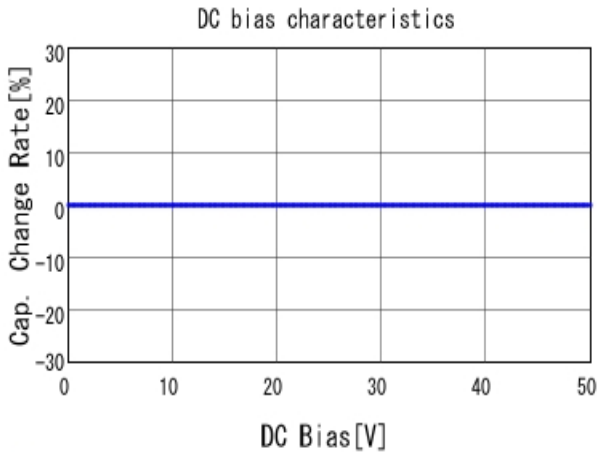
■ GRM0225C1H4R4CA03 C-DC bias capchange, 25.0degC, AC1V
