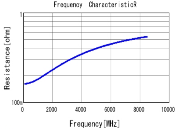
■ GRM0225C1H4R4CA03 R DC0V, 25degC
