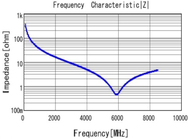
■ GRM0225C1H4R4CA03 |Z| DC0V, 25degC
