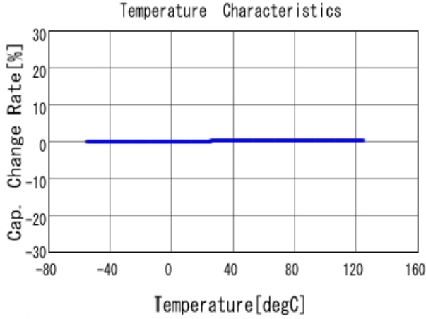
■ GRM0225C1H4R4CA03 C-Temp. capchange, DCOV, AC1Vrms
