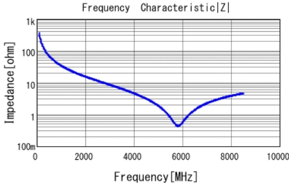
■ GRM0225C1H4R5WA03 |Z| DCOV, 25degC
