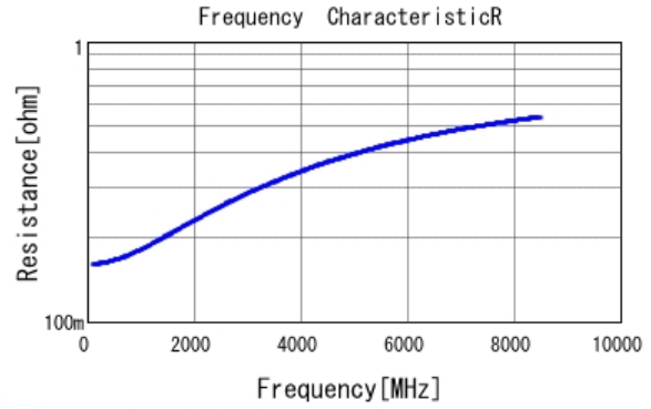
■ GRM0225C1H4R5WA03 R DCOV, 25degC
