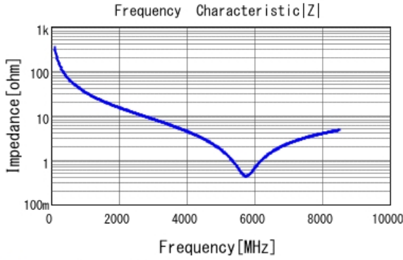
■ GRM0225C1H4R6CA03 |Z| DCOV, 25degC
