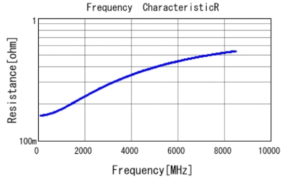
■ GRM0225C1H4R6CA03 R DCOV, 25degC
