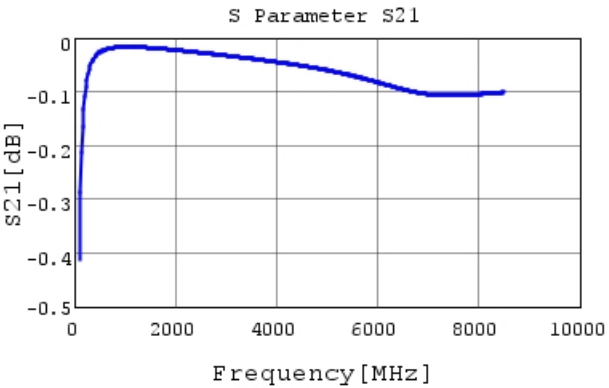
GRM0225C1H510JA02 S21 DCOV, 25degC
