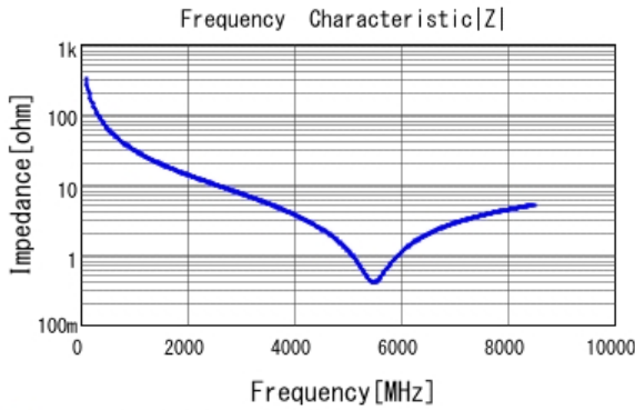
■ GRM0225C1H5R0CA03 |Z| DCOV, 25degC
