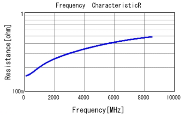
■ GRM0225C1H5R0CA03 R DCOV, 25degC
