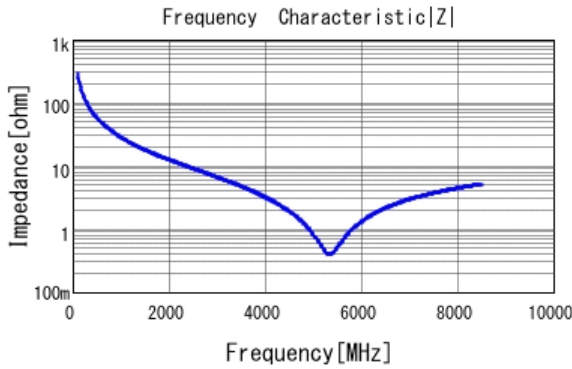
■ GRM0225C1H5R4BA03 |Z| DCOV, 25degC
