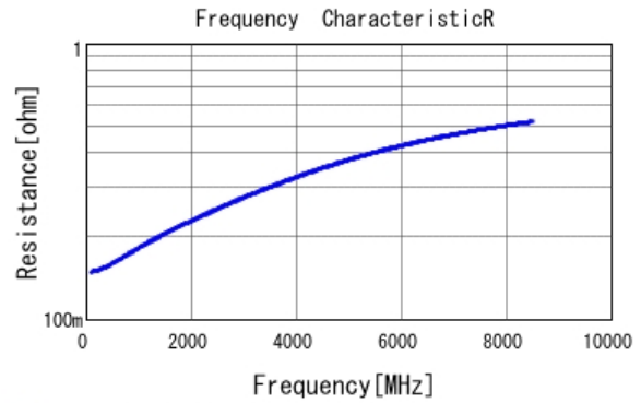
■ GRM0225C1H5R4BA03 R DCOV, 25degC
