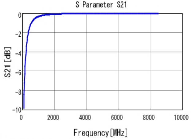
■ GRM0225C1H5R4WA03 S21 DCOV, 25degC
