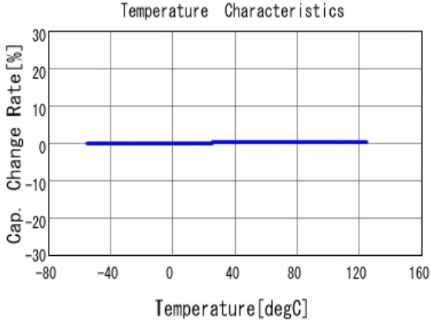
■ GRM0225C1H5R4WA03 C-Temp. capchange, DCOV, AC1Vrms
