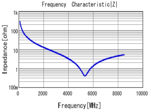
■ GRM0225C1H5R4WA03 |Z| DC0V, 25degC
