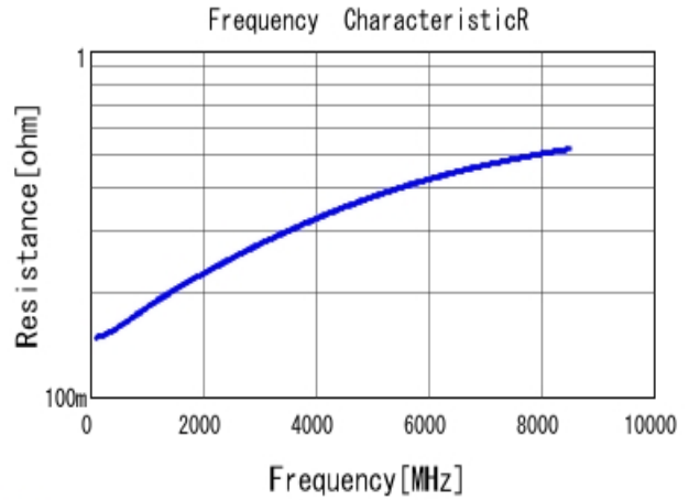
■ GRM0225C1H5R4WA03 R DC0V, 25degC
