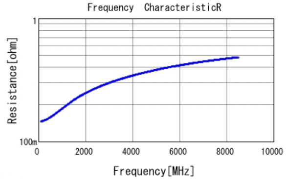
■ GRM0225C1H5R6CA03 R DCOV, 25degC
