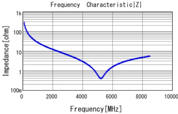
■ GRM0225C1H5R6CA03 |Z| DCOV, 25degC
