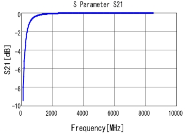
■ GRM0225C1H5R7BA03 S21 DCOV, 25degC
