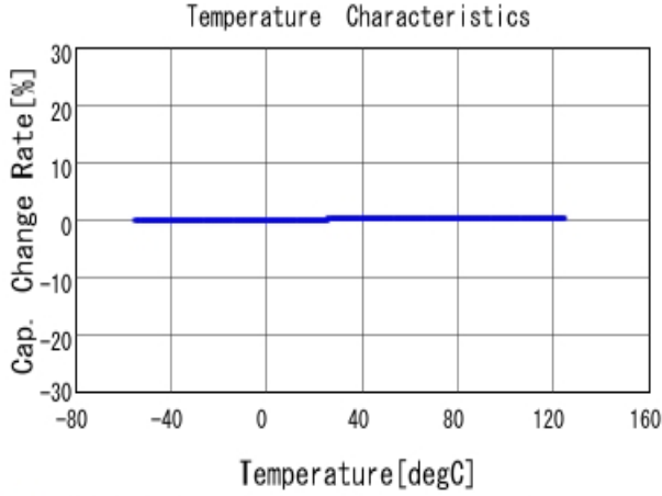
■ GRM0225C1H5R7BA03 C-Temp. capchange, DCOV, AC1Vrms
