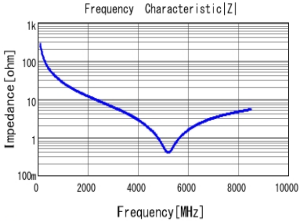
■ GRM0225C1H5R7BA03 |Z| DC0V, 25degC
