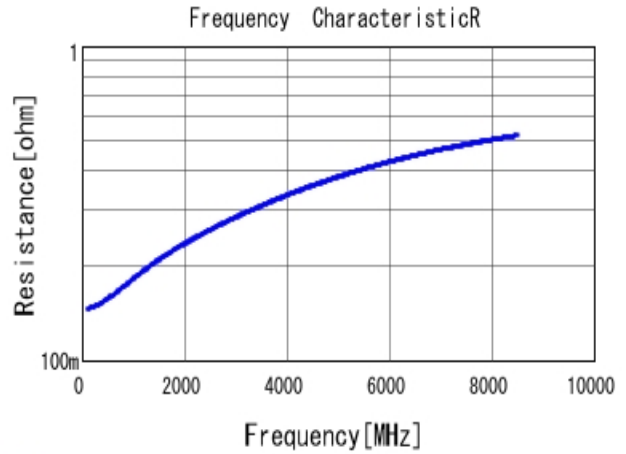
■ GRM0225C1H5R7BA03 R DC0V, 25degC
