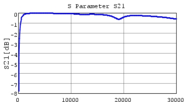
GRM0225C1H7R1WA03 S21 DCOV, 25degC
