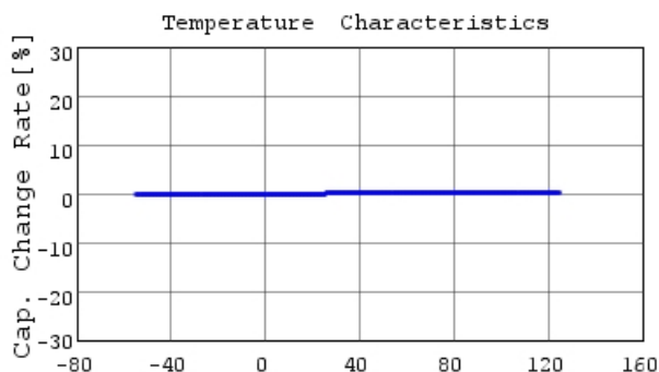
GRM0225C1H7R1WA03 C-Temp. capchange, DCOV, 1
