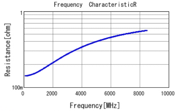
■ GRM0225C1H7R2BA03 R DCOV, 25degC
