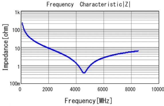
■ GRM0225C1H7R2BA03 |Z| DCOV, 25degC
