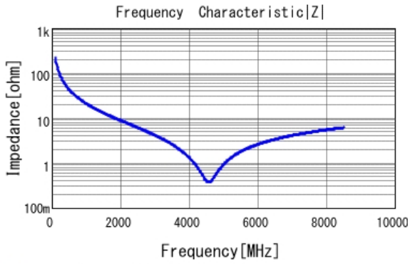
■ GRM0225C1H7R2DA03 |Z| DCOV, 25degC
