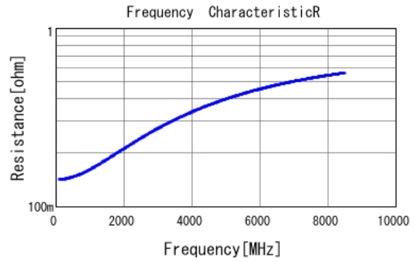
■ GRM0225C1H7R2DA03 R DCOV, 25degC
