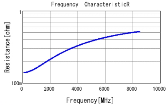
■ GRM0225C1H7R4BA03 R DC0V, 25degC
