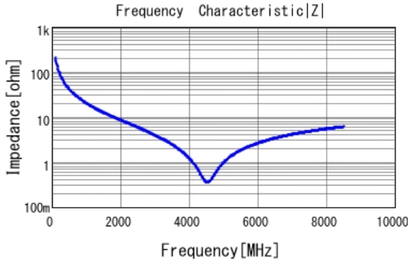
■ GRM0225C1H7R4BA03 |Z| DC0V, 25degC
