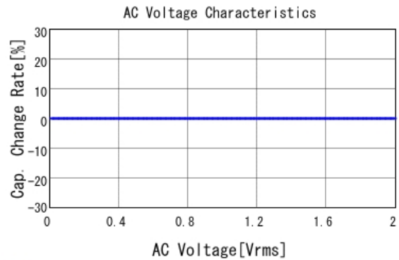
■ GRM0225C1H7R4BA03 C-AC Voltage capchange, DC0V, 25.0d
