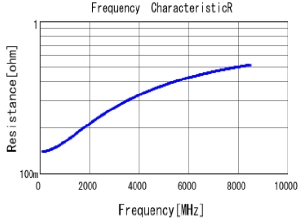
■ GRM0225C1H7R5BA03 R DC0V, 25degC
