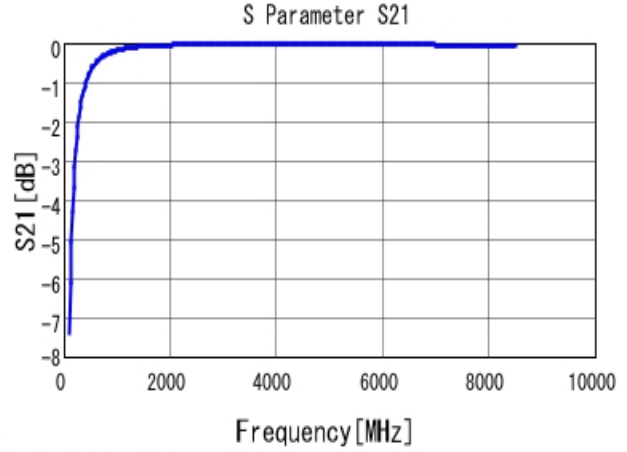
■ GRM0225C1H7R5BA03 S21 DCOV, 25degC
