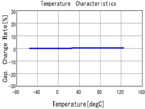
■ GRM0225C1H7R5BA03 C-Temp. capchange, DCOV, AC1Vrms
