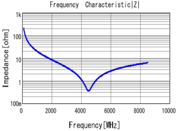
■ GRM0225C1H7R5BA03 |Z| DC0V, 25degC
