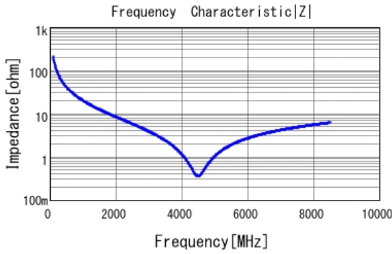
■ GRM0225C1H7R5DA03 |Z| DC0V, 25degC
