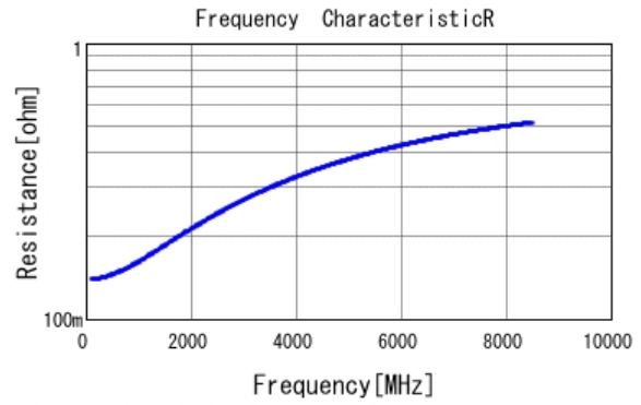
■ GRM0225C1H7R5DA03 R DC0V, 25degC
