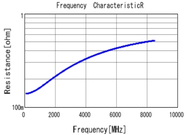
■ GRM0225C1H7R6WA03 R DC0V, 25degC
