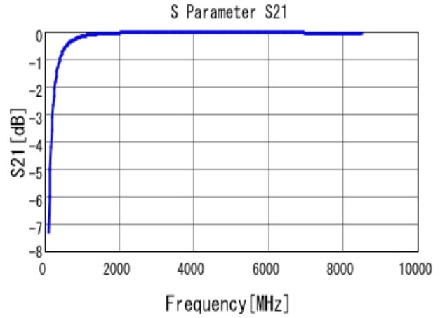
■ GRM0225C1H7R6WA03 S21 DCOV, 25degC
