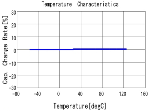
■ GRM0225C1H7R6WA03 C-Temp. capchange, DCOV, AC1Vrms
