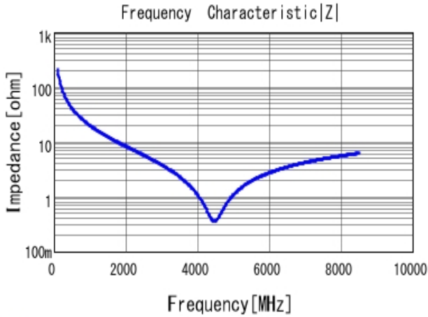
■ GRM0225C1H7R6WA03 |Z| DC0V, 25degC
