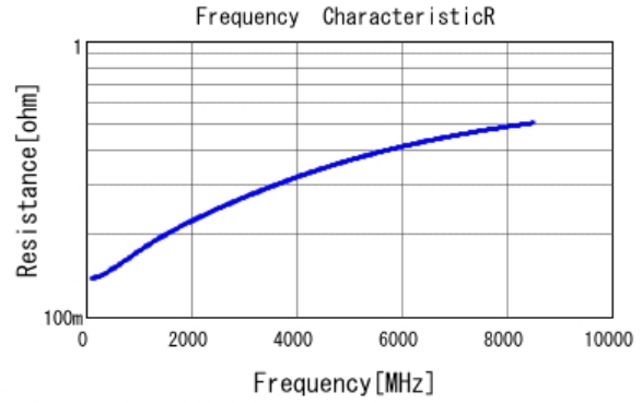
■ GRM0225C1H7R7BA03 R DCOV, 25degC
