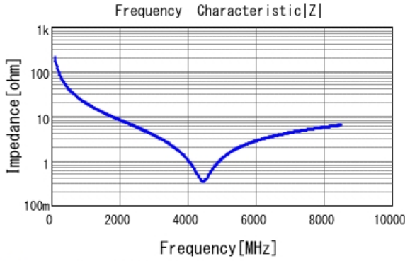
■ GRM0225C1H7R7BA03 |Z| DCOV, 25degC
