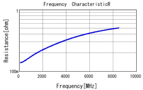
■ GRM0225C1H7R9BA03 R DC0V, 25degC
