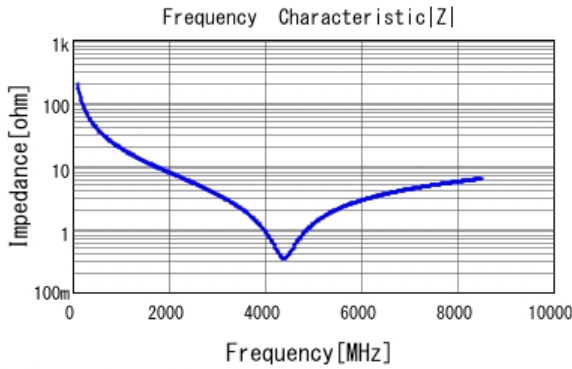
■ GRM0225C1H7R9BA03 |Z| DC0V, 25degC
