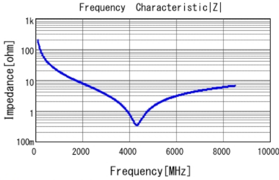
■ GRM0225C1H8R0DA03 |Z| DCOV, 25degC
