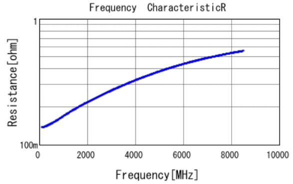
■ GRM0225C1H8R0DA03 R DCOV, 25degC
