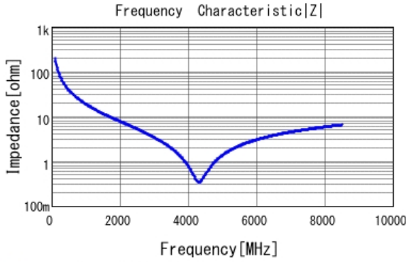
■ GRM0225C1H8R0WA03 |Z| DCOV, 25degC
