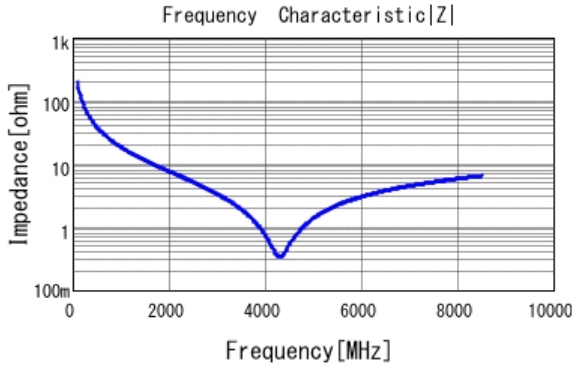
■ GRM0225C1H8R1WA03 |Z| DCOV, 25degC
