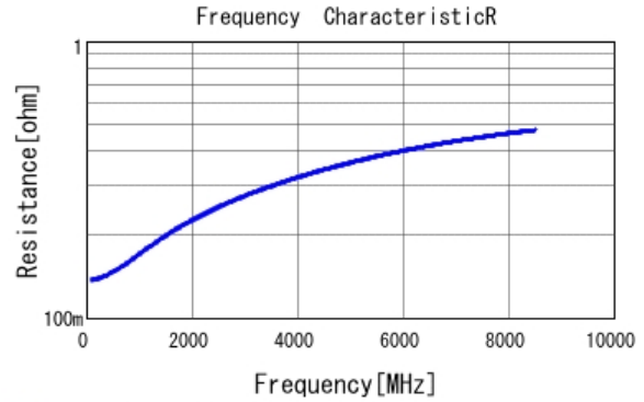
■ GRM0225C1H8R1WA03 R DCOV, 25degC
