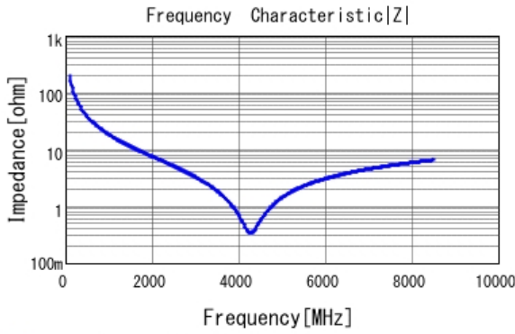
■ GRM0225C1H8R2DA03 |Z| DCOV, 25degC
