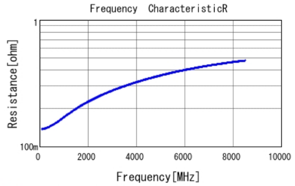
■ GRM0225C1H8R2DA03 R DCOV, 25degC
