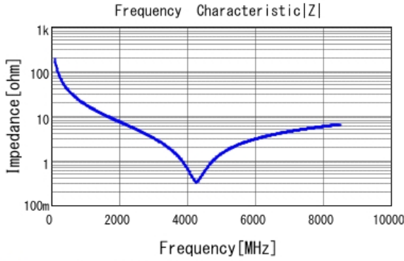
■ GRM0225C1H8R3BA03 |Z| DCOV, 25degC
