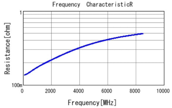
■ GRM0225C1H8R3BA03 R DCOV, 25degC
